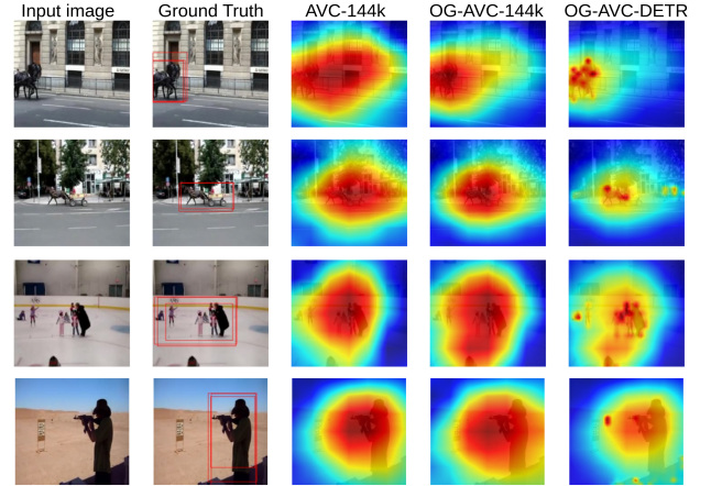
Figure 3: Localization maps for our variants: AVC-144k (student model), OG-AVC (object-guided AVC-144k), and OG-AVC-DETR (AVC-144k with ResNet18 and DETR predictions). Trained on Flickr-144k, samples from test set.
