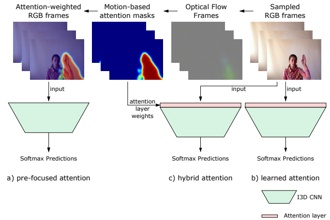
Fig. 1. Overview of the proposed methods. The top part shows the steps for generating the attention-weighted RGB frames. The inputs used for the three proposed methods are then depicted.
