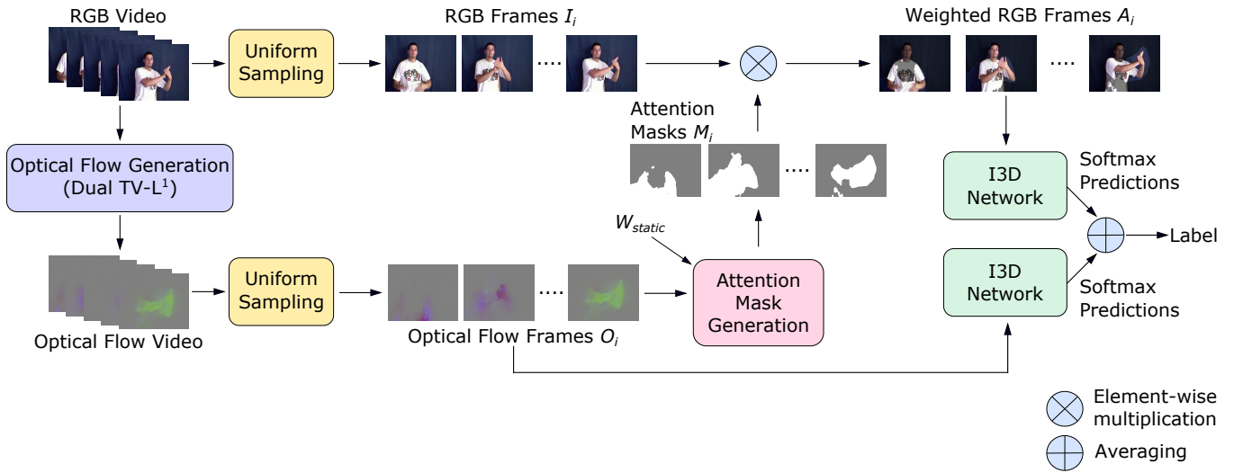
Fig. 2. Pre-focused Attention Architecture. A motion prior focuses attention on regions of interest via Attention Masks. The general network architecture consists of two streams of I3D networks [4]. The first (upper) one is fed weighted RGB frames, and the second (lower) one takes optical flow frames as input, which have been computed using the Dual-TV L algorithm [54]. The weighted RGB frames are computed by generating attention masks from the optical flow frames and multiplying them element-wise with the RGB frames. The two I3D Networks generate predictions of the presented gesture and are finally averaged to yield a final label (details of the I3D network in Fig. 3).
