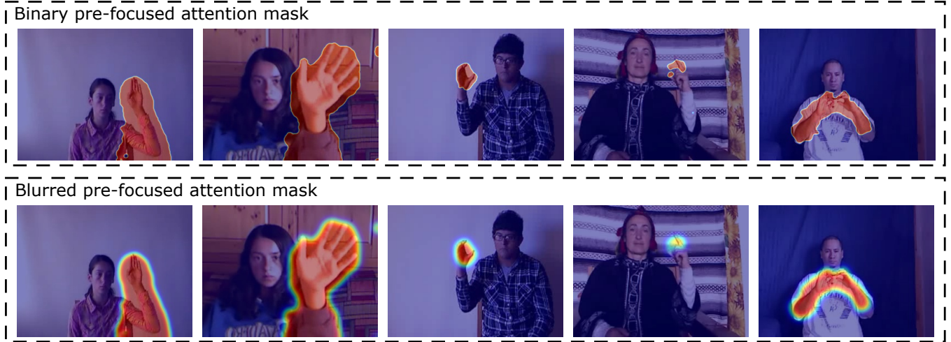
Fig. 4. Visualization of Pre-focused Attention Maps. An example of attention-weighted RGB frames from ChaLearn249 dataset [45] after applying pre-focused attention to the RGB frame. Top: binary masks, where the red areas represent motion-based attention areas and the blue areas show no motion, therefore less attention. Bottom: Blurring out the mask to allow for a smoother transition between the focus areas and the surrounding areas.
